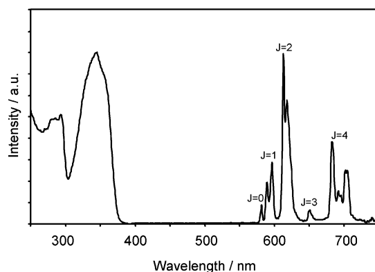
FIGURE 1. Corrected excitation (250–450 nm, \lambda_{em} = 618 nm) and emission (550–750 nm, \lambda_{ex} = 349 nm) spectra of the Eu- 6 complex solution (1 × 10 -6 M in borate buffer, pH 8.6). Excitation and emission band-passes 2.5 nm, delay time 0.1 ms, gate time 0.4 ms. The emission bands arise from the 5 D 0 → 7 F J transitions; the J values are shown on the spectrum.
